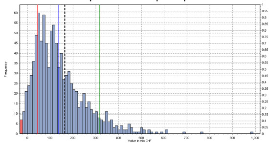
Figure 4: Value Distribution for Pharma
