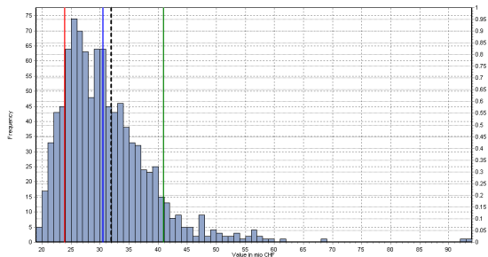
Figure 3: Value Distribution for Bio-Tec
