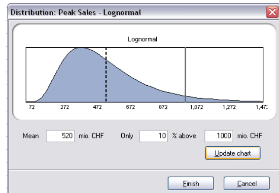
Figure 2: Peak sales are lognormally distributed
